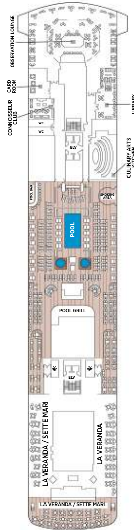
DECK 11
